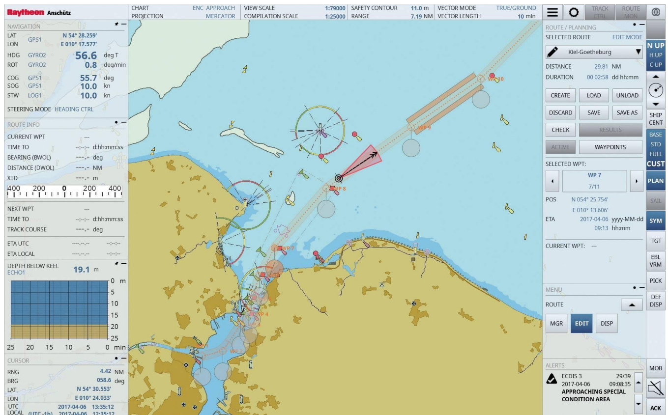
ECDIS monitor (Electronic Chart Display and Information System)
